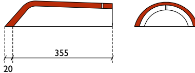
uni-hoekkeperbeginvorst
