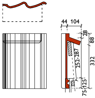
chaperonpan 70°
